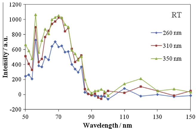
Fig. 5. Excitation spectra of CsCaCl 3 .
