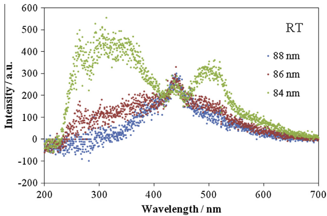
Fig. 4. Luminescence spectra of CsCaCl 3 for excitation at 84–88 nm.
