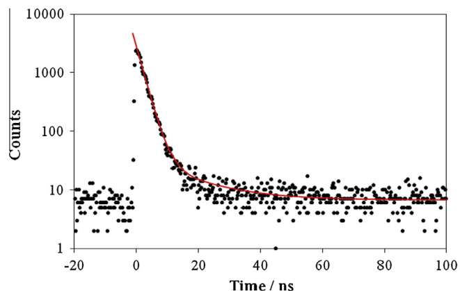
Fig. 8. Scintillation time profile of \text{CsCaCl}_3 . The solid line represents the fitted function.
