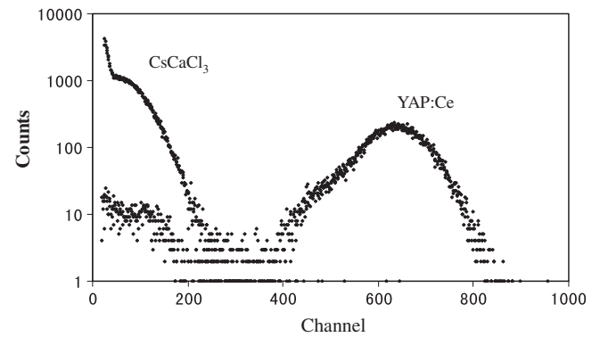
Fig. 7. Pulse-height spectra of scintillation detectors equipped with a CsCaCl 3 or a YAlO 3 :Ce (YAP:Ce) crystal for 67.4 keV X-ray. Note that the amplifier gain was ten times smaller for YAP:Ce.
