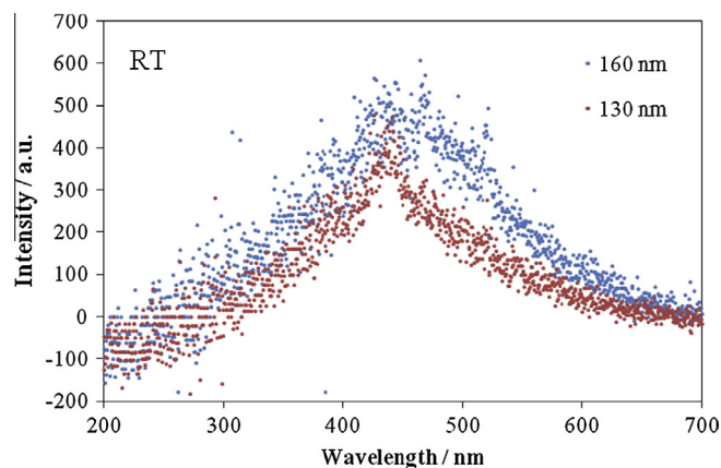
Fig. 3. Luminescence spectra of CsCaCl 3 for the excitation at 160 and 130 nm.
