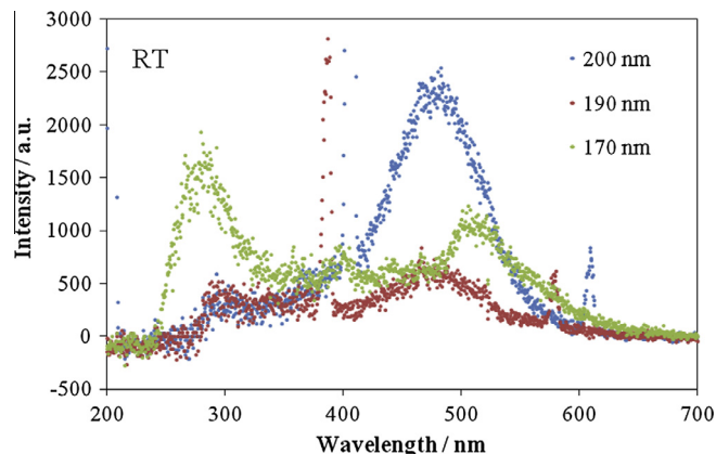
Fig. 2. Luminescence spectra of CsCaCl 3 for the excitation at 170–200 nm.
